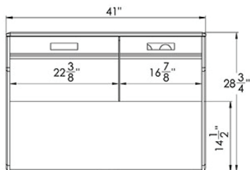
Dual Wedge/Pod Configuration Shown
